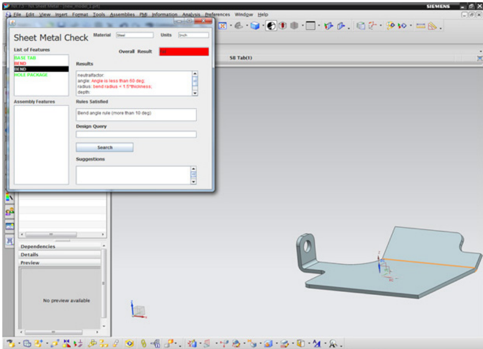
Fig. 18. Integrating rule checking within a CAD design tool.
